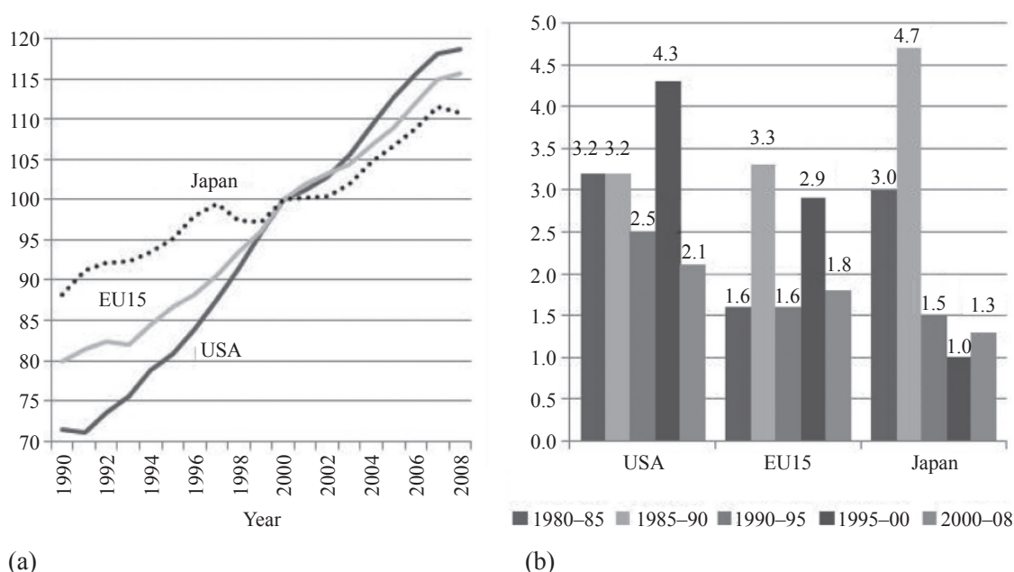
Figure 2. (a) Long-term GDP growth trends: EU15, Japan, USA (volume index; 2000 = 100), and (b) % change per year, 1980–2008 (source: authors' own calculations based on OECD, 2010).
